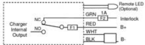
Figure 2: Charger Connections
